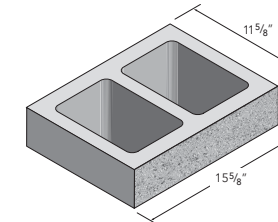
12x4x16 Standard
