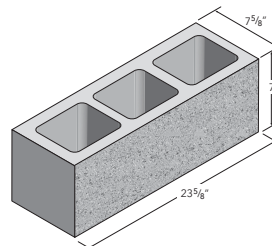
8x8x24 Standard
