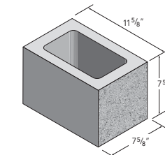
12x8x8 Standard
