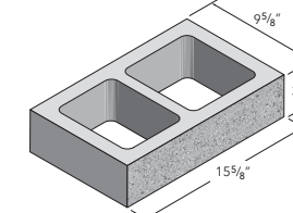
10x4x16 Standard
