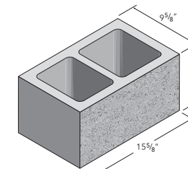
10x8x16 Standard
