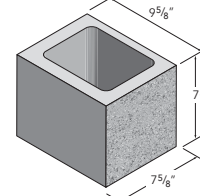
10x8x8 Standard
