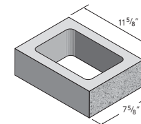
12x4x8 Standard
