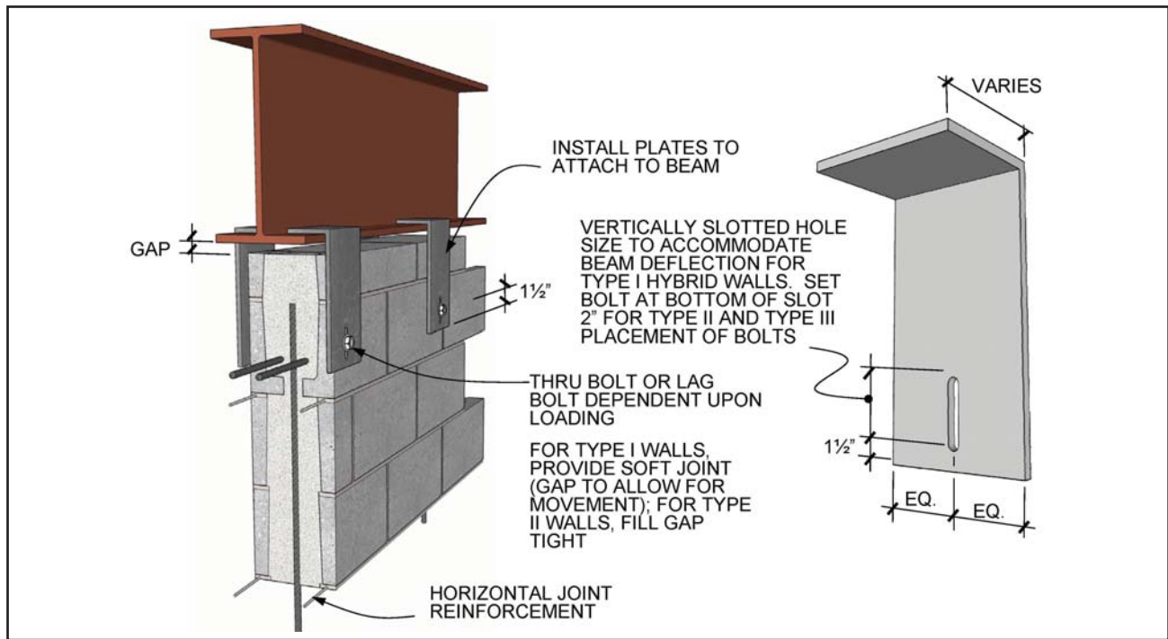
Figure 5A—Connector Plate Detail
