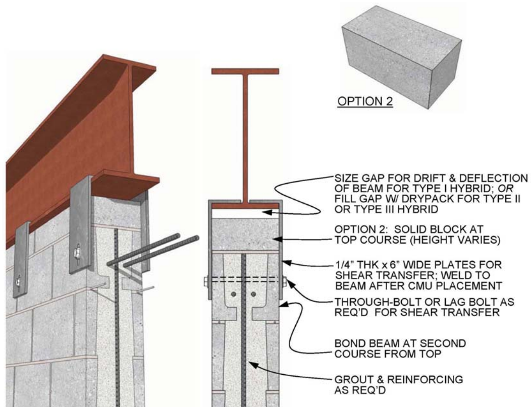
Figure 5—Top of Wall Details
