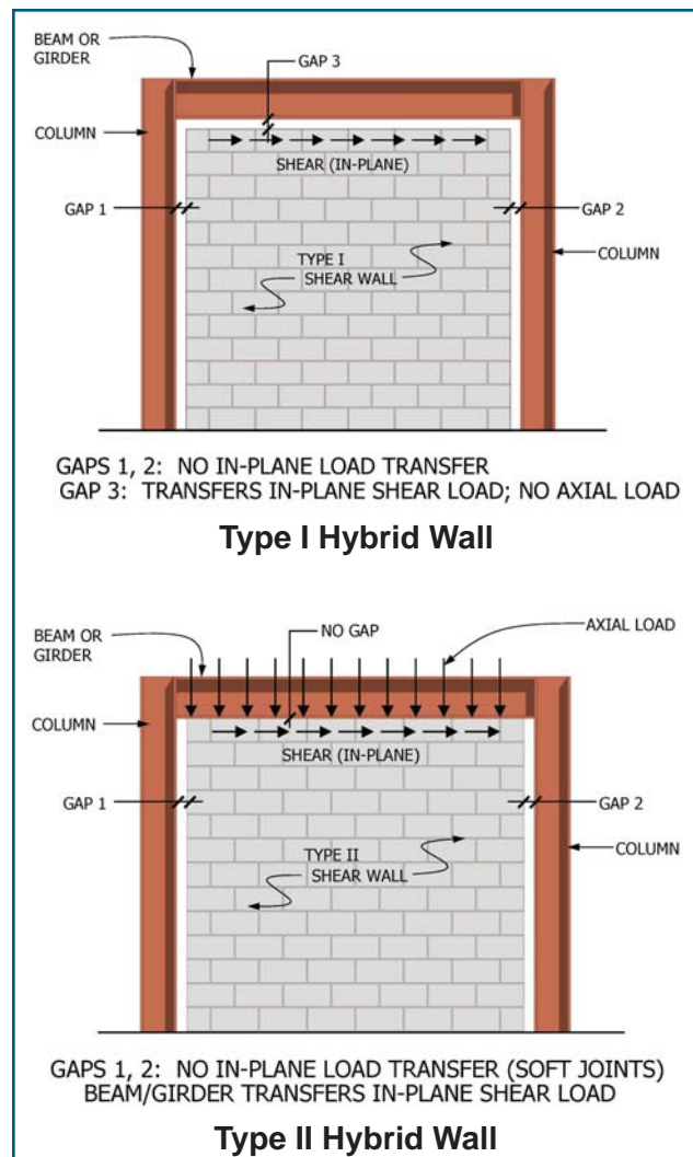
Figure 1—Hybrid Wall Types I and II
