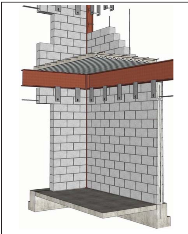
Figure 2—Type I and IIa Foundation and Floor Detail
