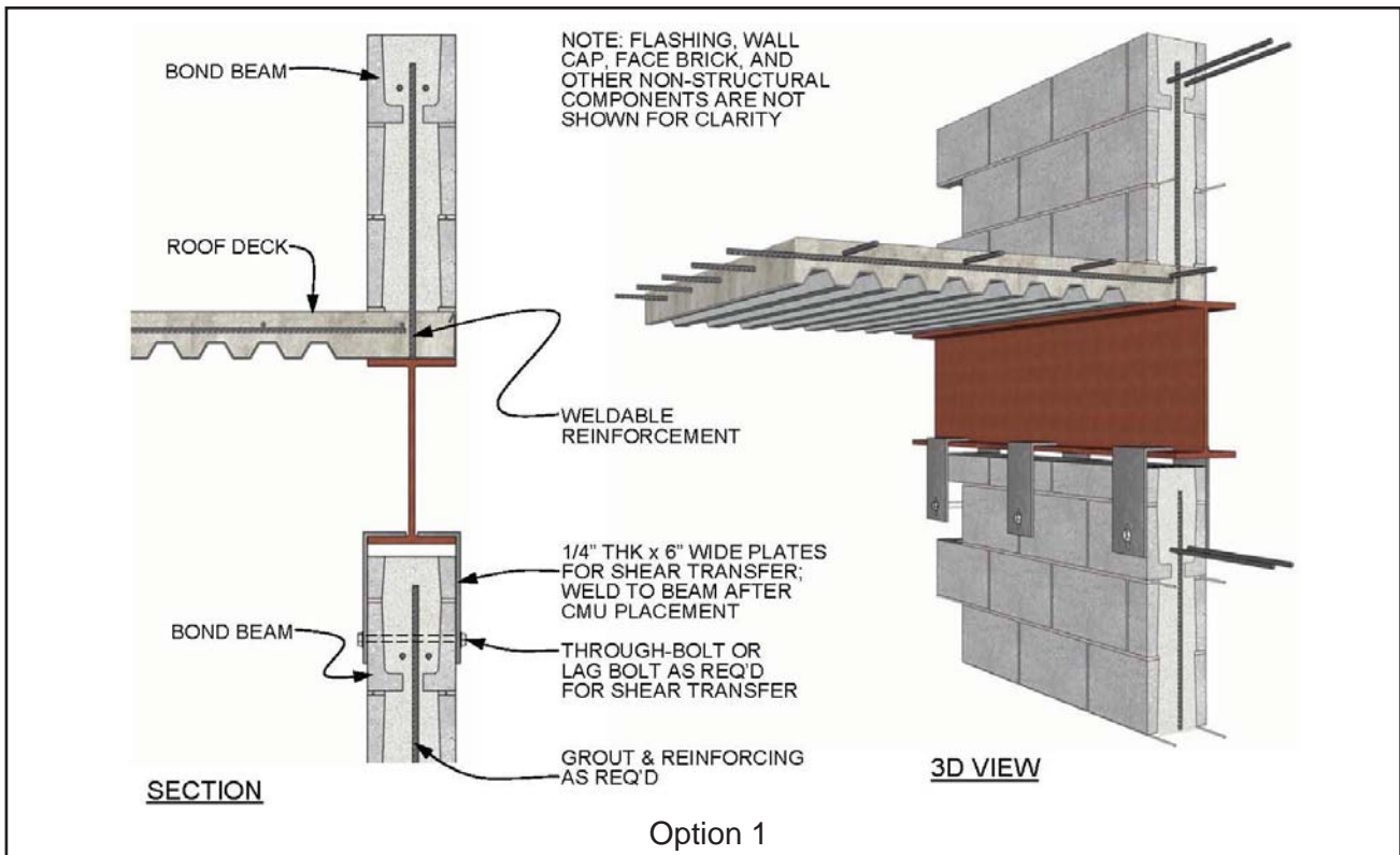
Figure 7—Parapet Details
