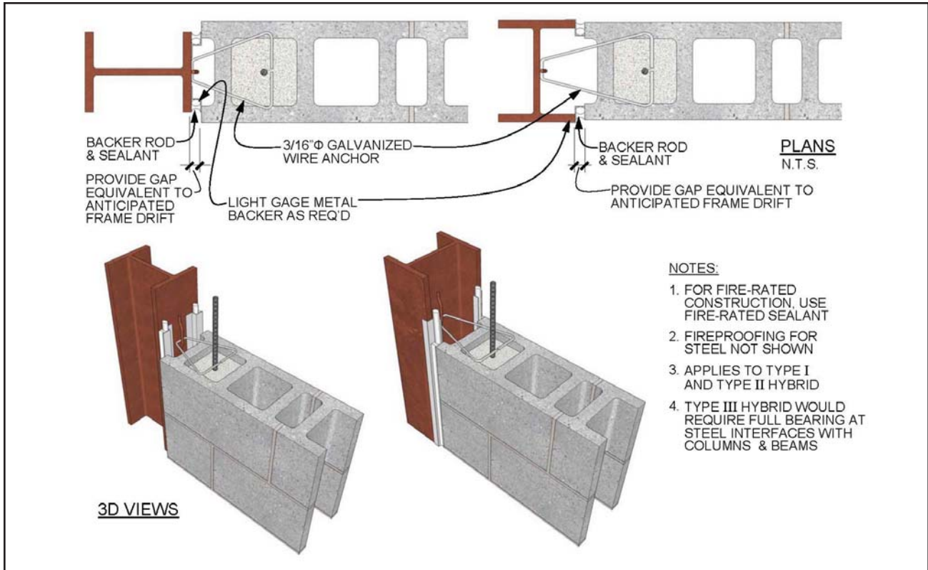
Figure 6—Column Details
