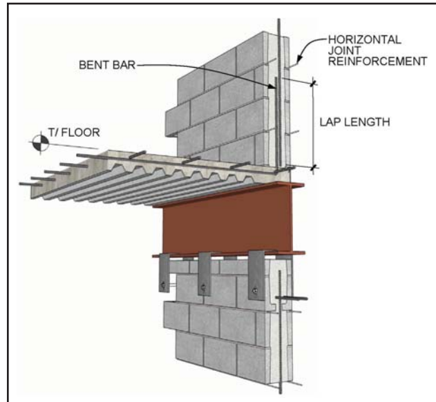
Figure 4—Type IIb Floor Detail
