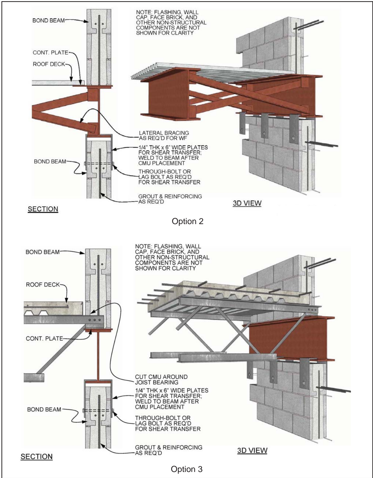
Figure 7—Parapet Details (continued)
