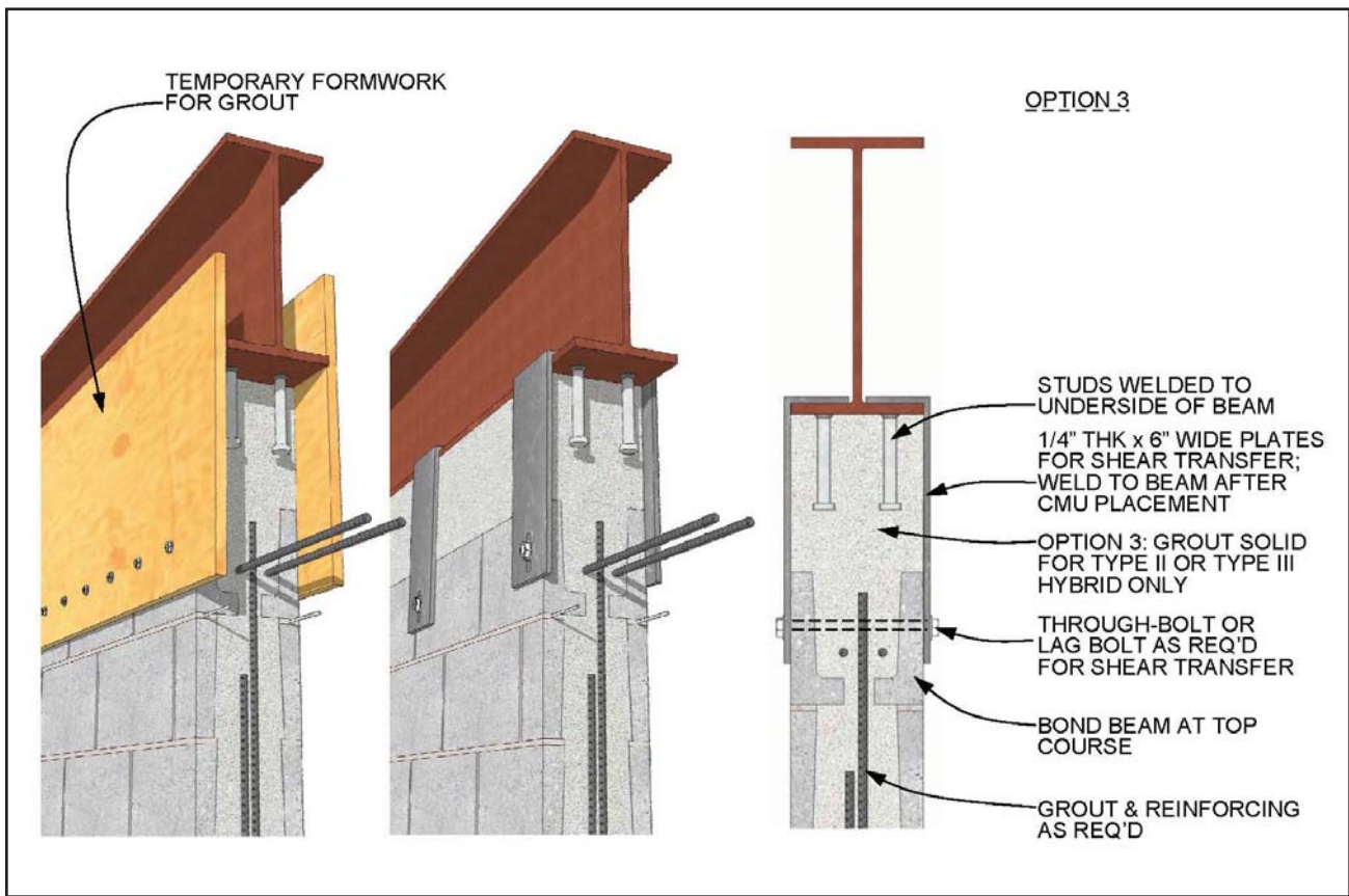
Figure 5—Top of Wall Details (continued)
