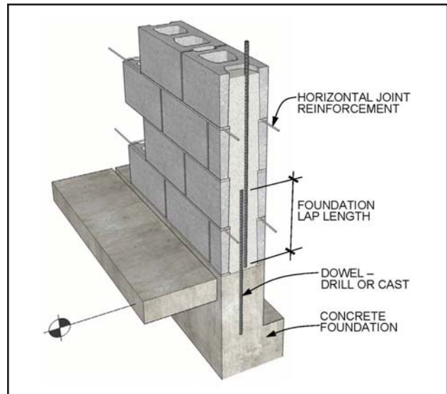
Figure 3—Type IIb Foundation Detail
